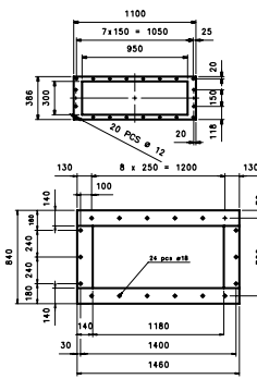
Rollermill inlet B-B
