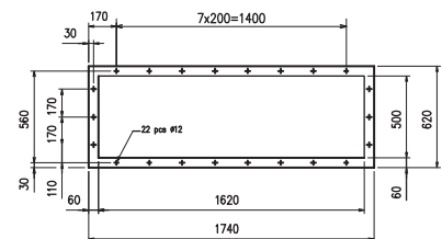
Crumbler bottom flange C-C
