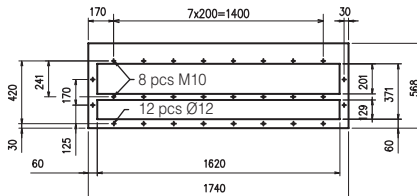
Crumbler top flange B-B
